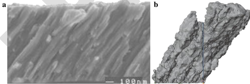
Figure 11: (a) SEM image of a GLAD coating (b) 3D mesh of a simulated PVD world
